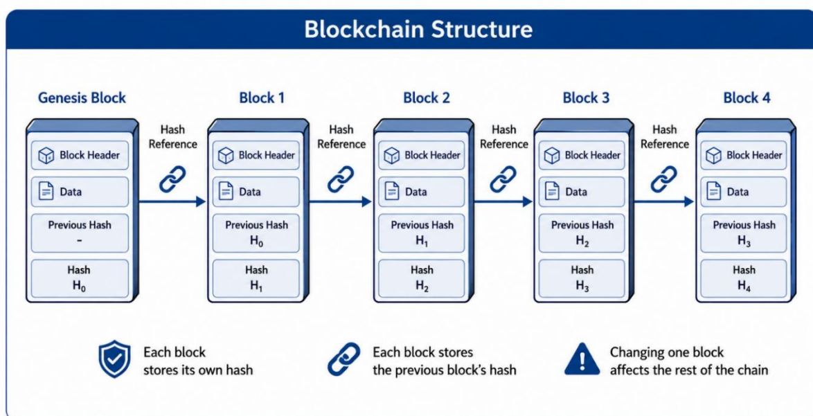
Fig. 4. Pictorial representation of chained blocks linked by cryptographic hash references.
